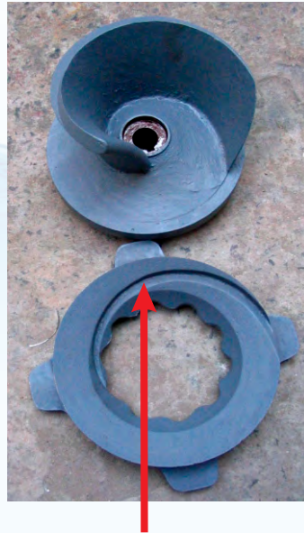
Self Cleaning & Cutting Spiral Groove : Centrifugally "sweeps" blockage causing fibres away from Impeller Casing Cover to Discharge Nozzle thereby keeping the pump clog free
